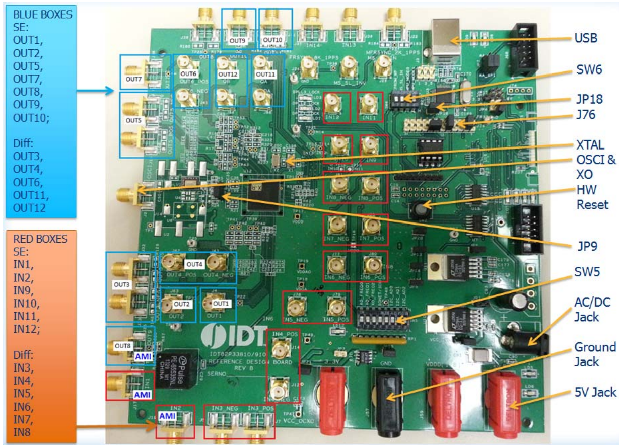
Figure 1. Board Overview
