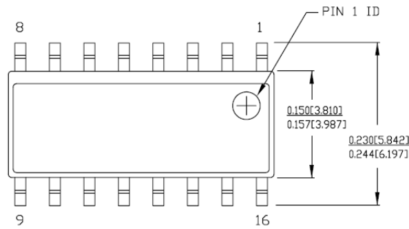
Figure 16. 16-Pin (150-Mil) SOIC
