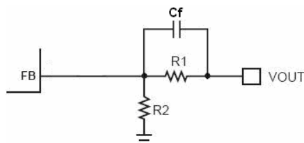
Figure 2—Feedback Network
