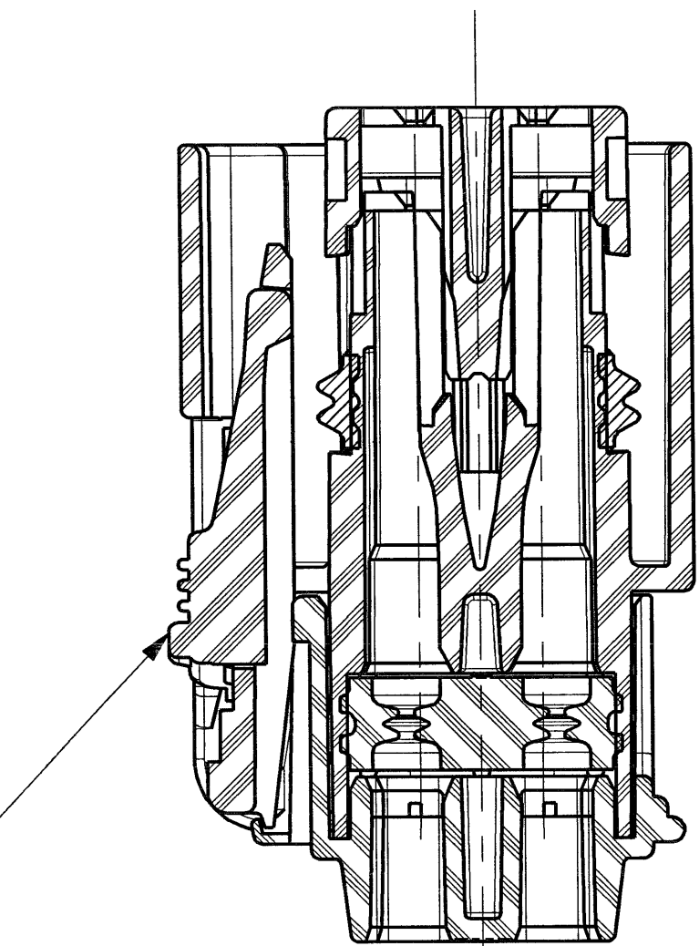
SECTION A-A C.P.A. & T.P.A. IN PRE-ASSEMBLED POSITION (SHOWN WITH OPTIONAL C.P.A.)
