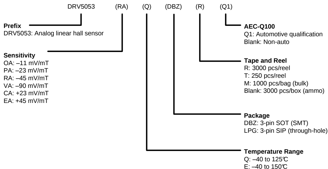
Figure 17. Device Nomenclature
