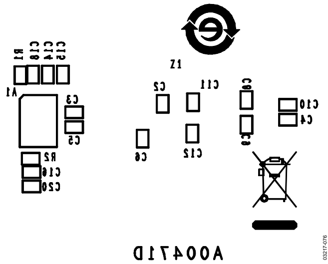
Figure 75. Wiring-Side Silkscreen
