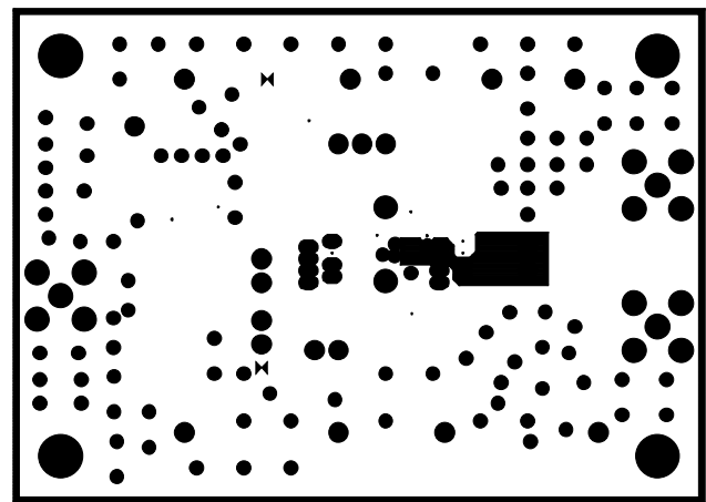
Figure 77. Inner Layer 2
