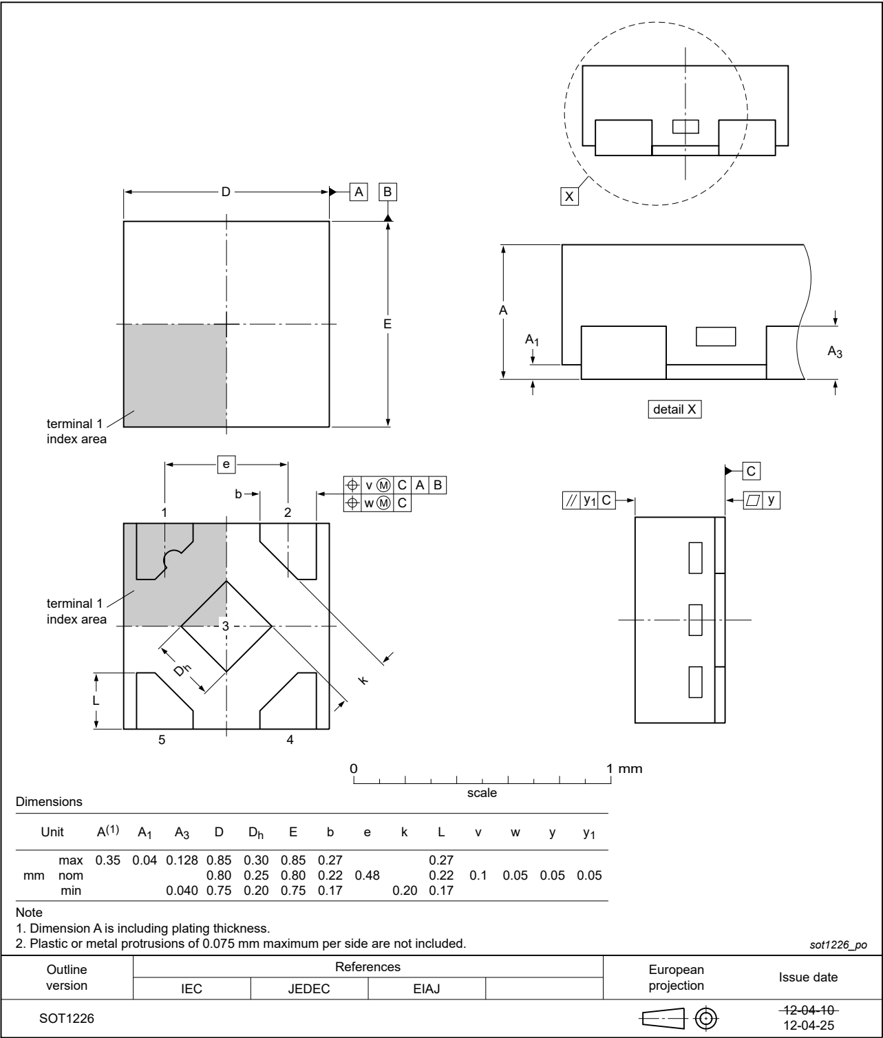
Fig. 11. Package outline SOT1226 (X2SON5)
