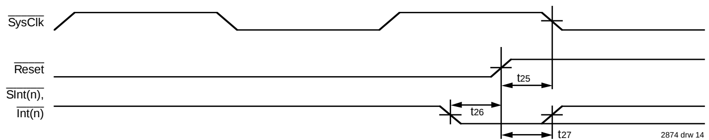
Figure 11. Mode Selection and Negation of Reset
