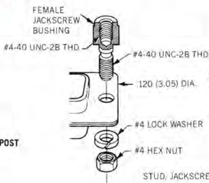
JACKPOST ASSEMBLY
