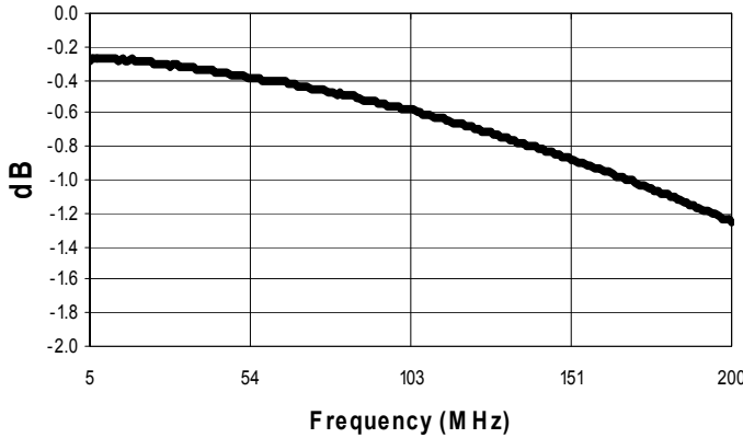
Insertion Loss 1 (Pin5 - Pin1)
