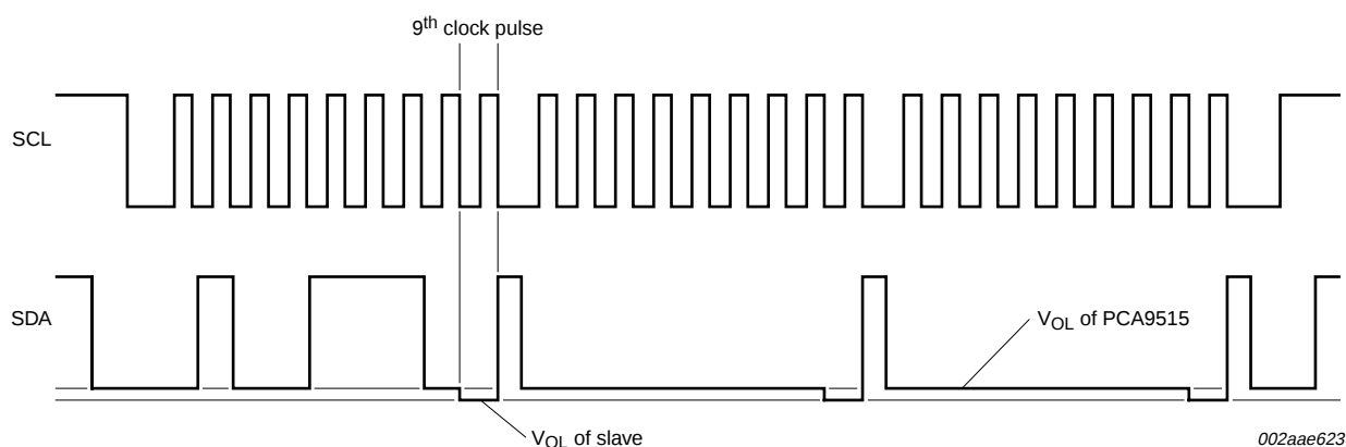
Fig 6. Bus 1 waveform
