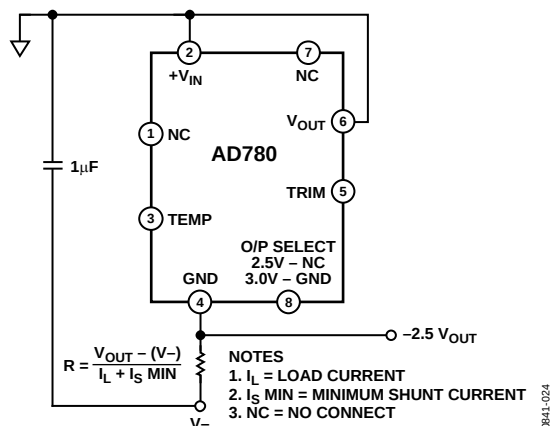
Figure 24. Negative (–2.5 V Shunt Mode Reference)
