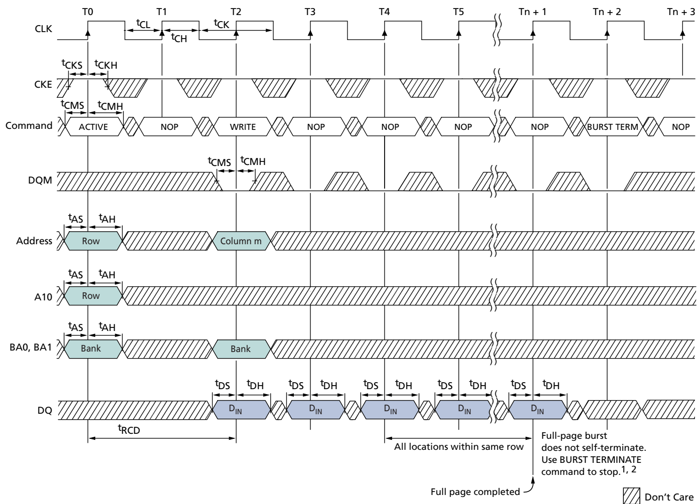
Figure 31: WRITE – Continuous Page Burst
