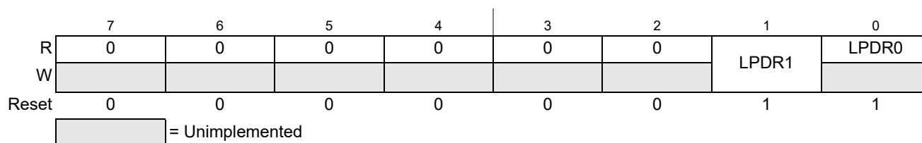
Figure 21-3. Port LP Data Register (LPDR)
