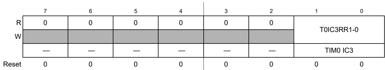
Figure 2-6. Module Routing Register 4 (MODRR4)
