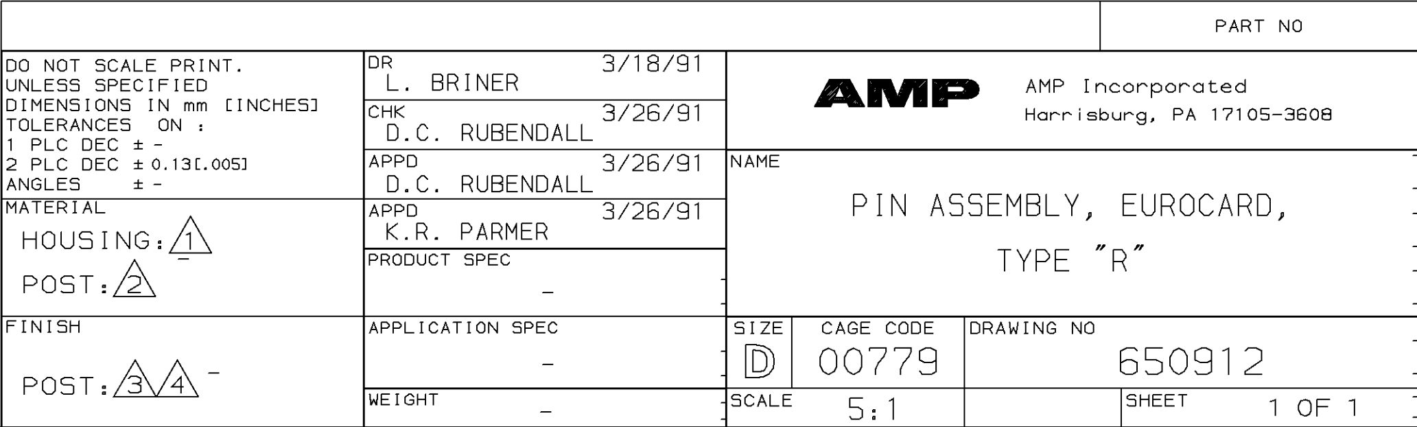
CUSTOMER DRAWING
