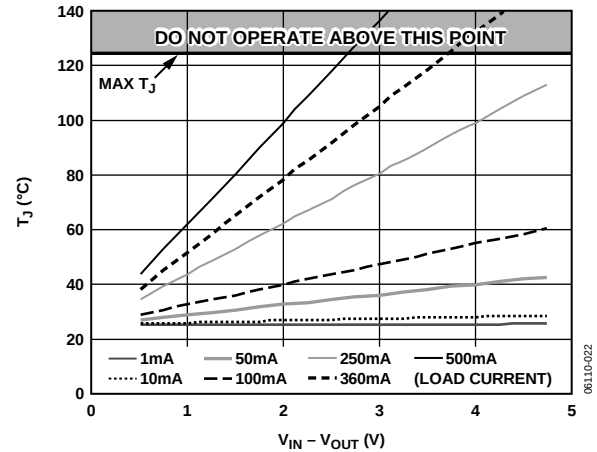
Figure 34. 700 mm² of PCB Copper, T_A = 25^\circ\text{C}
