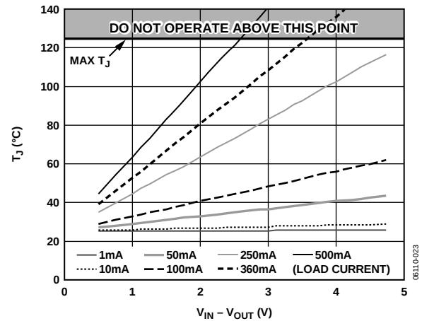
Figure 35. 300 mm² of PCB Copper, T_A = 25^\circ\text{C}
