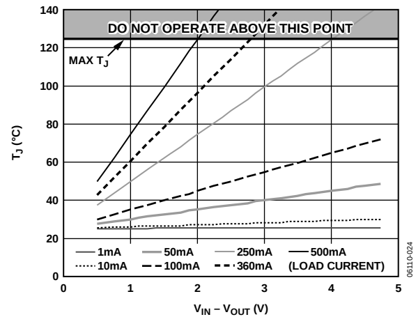
Figure 36. 100 mm² of PCB Copper, T_A = 25^\circ\text{C}
