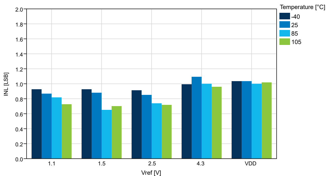
Figure 39-44. INL vs. V_{ref} ( V_{DD}=5.0 V, f_{ADC}=115 kps), REFSEL = Internal Reference
