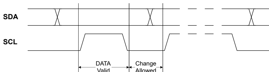
Figure 27-5. Data Validity
