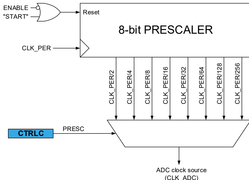
Figure 31-6. ADC Prescaler
