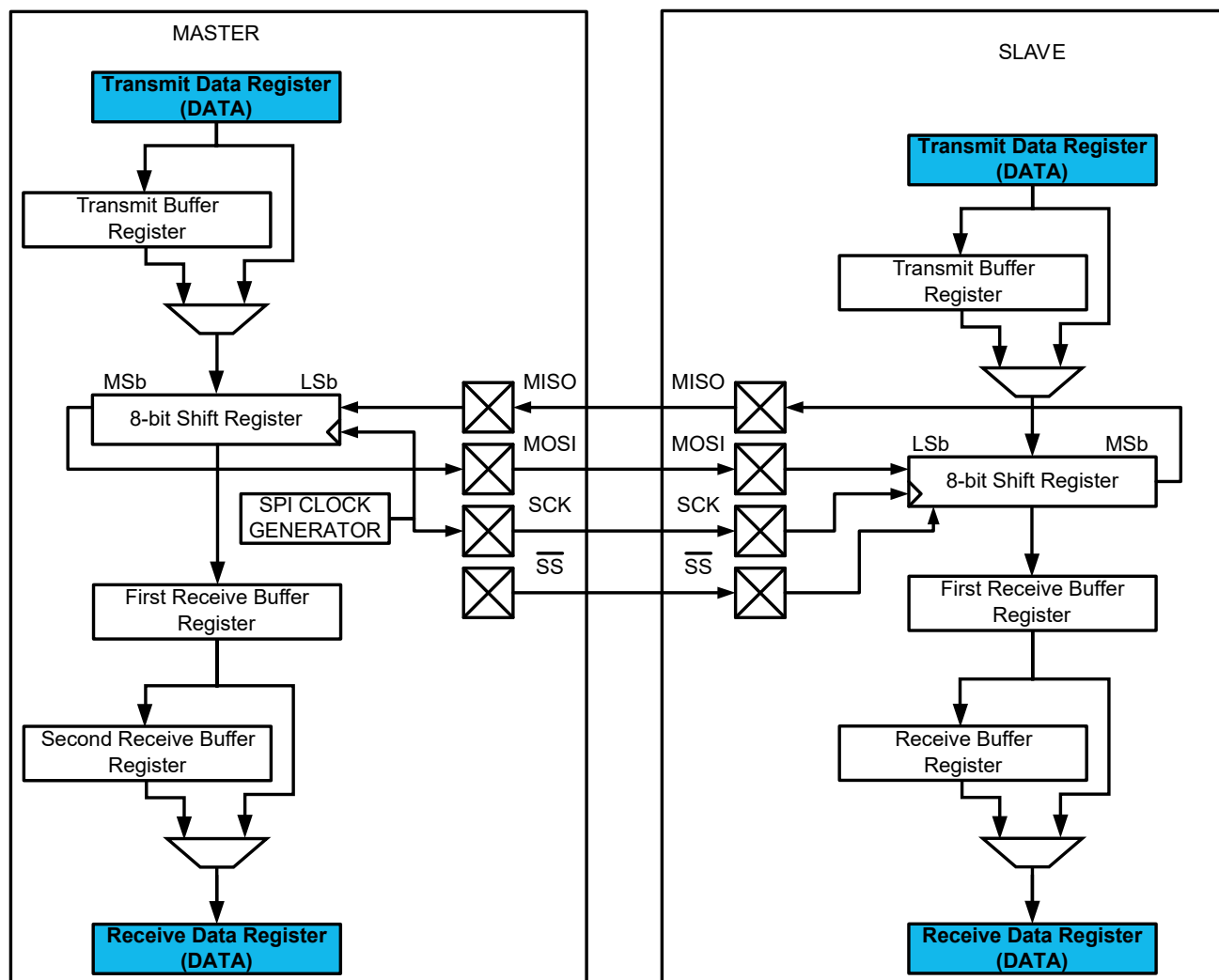
Figure 26-1. SPI Block Diagram
