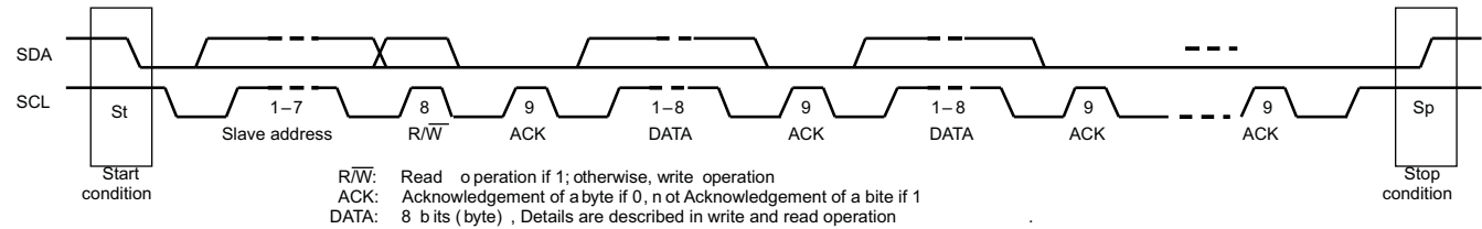
Figure 23. I²C Packet Protocol
