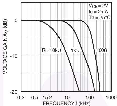
Fig. 16 Frequency Response
