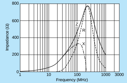
BLA31BD471SN4
