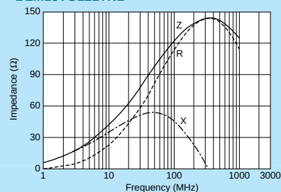
BLM18TG121TN1
