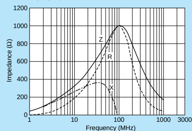
BLM18TG102TN1
