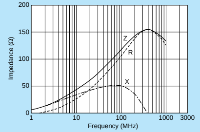
BLA31AG121SN4
