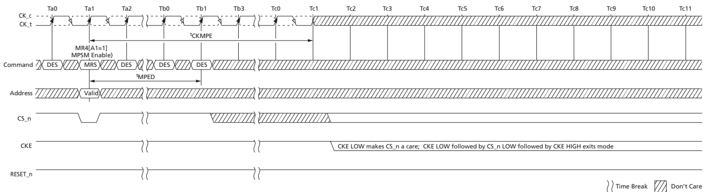
Figure 40: Maximum Power-Saving Mode Entry
