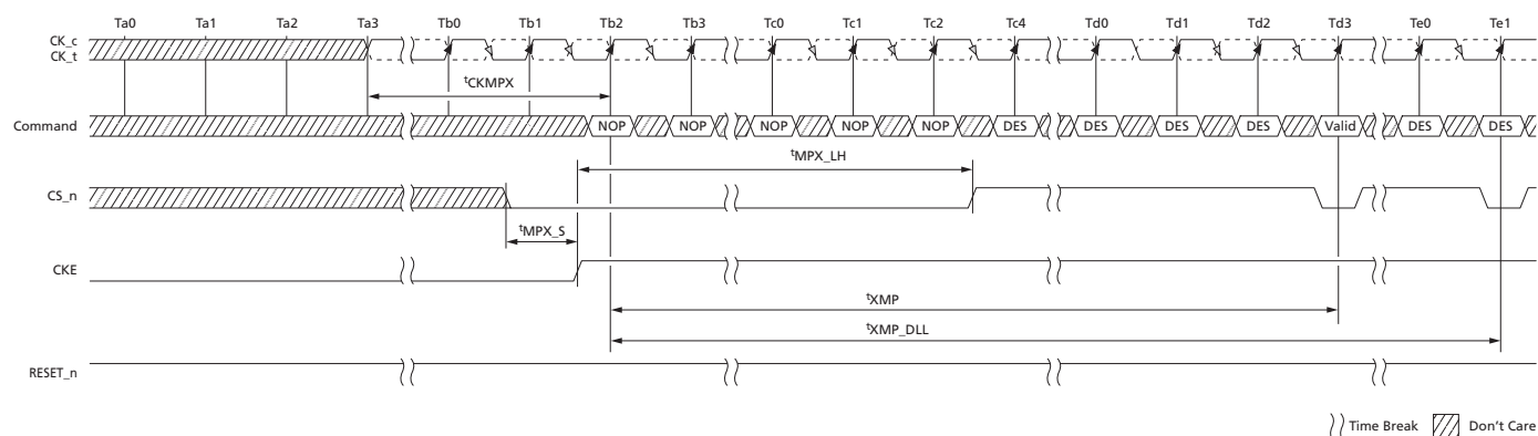
Figure 43: Maximum Power-Saving Mode Exit
