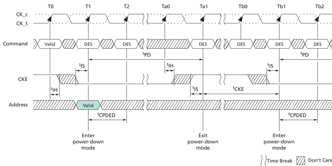
Figure 94: Power-Down Entry/Exit Clarifications – Case 1
