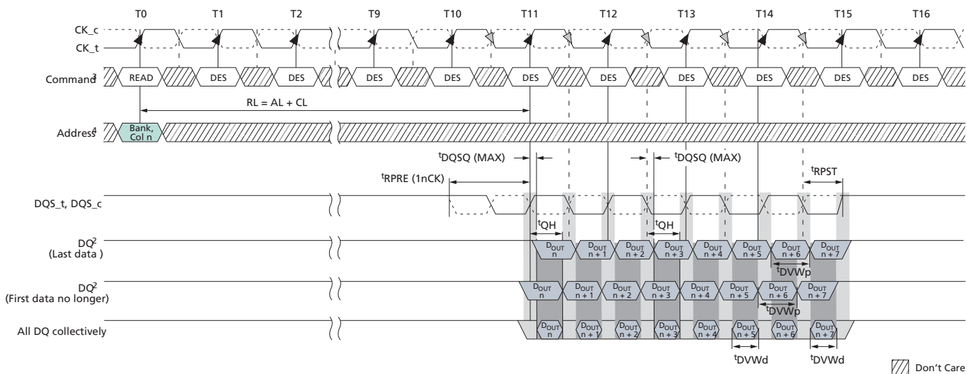
Figure 118: Data Strobe-to-Data Relationship
