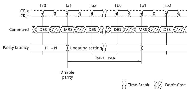
Figure 52: Parity Exit Timing Example – t_{MRD\_PAR}
