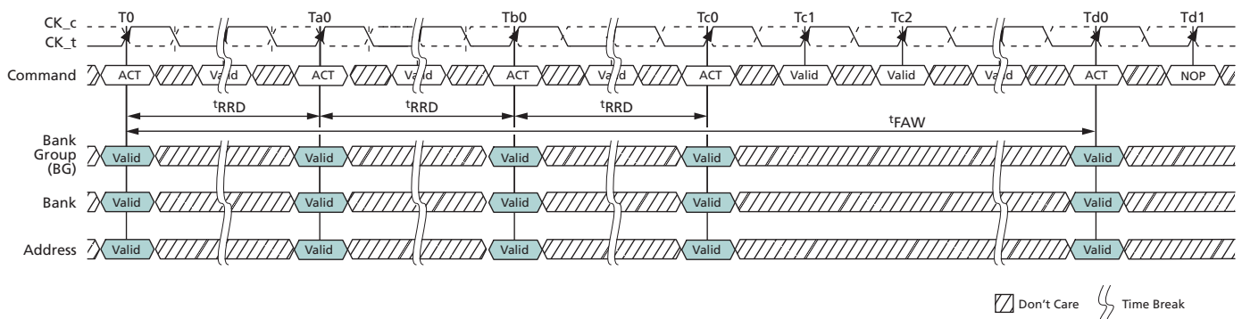
Figure 74: t_{FAW} Timing
