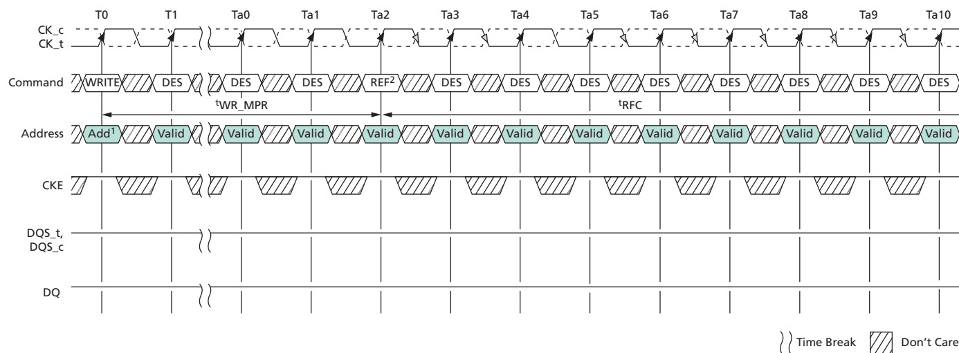
Figure 36: WRITE-to-REFRESH Timing
