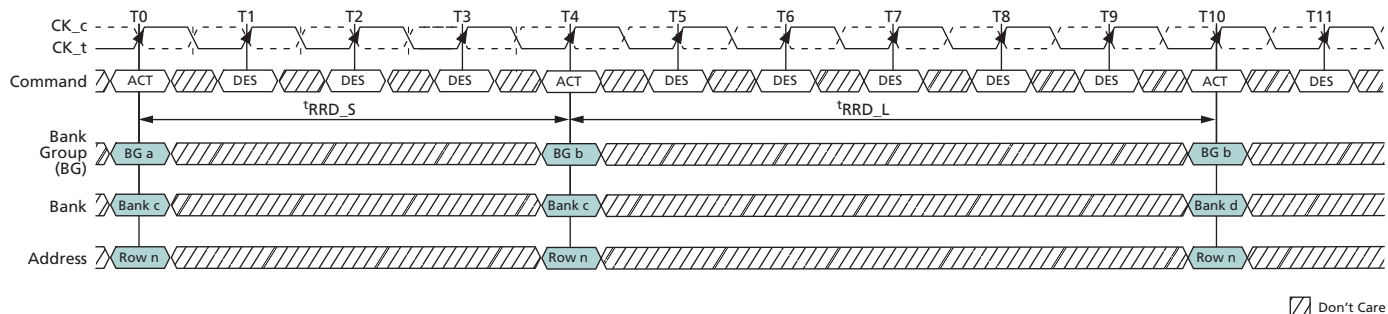
Figure 113: t_{RRD} Timing
