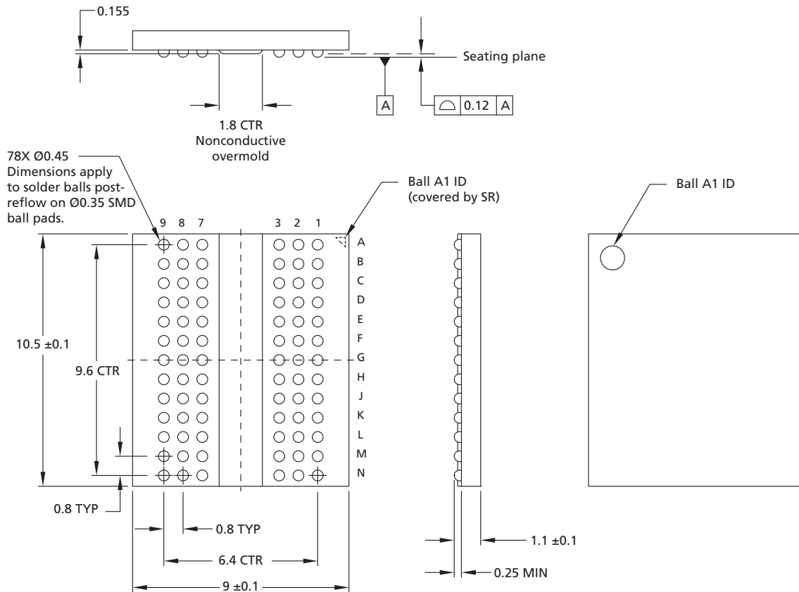
Figure 4: 78-Ball FBGA – x4, x8 "RH"
