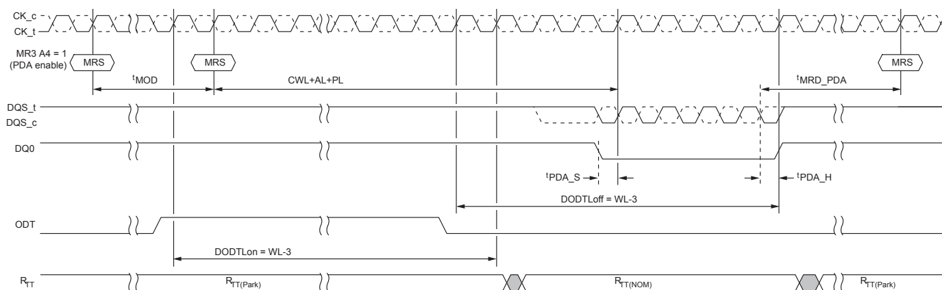
Figure 55: PDA Operation Enabled, BL8
