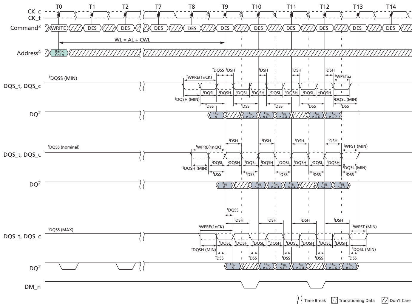
Figure 156: Write Timing Definition
