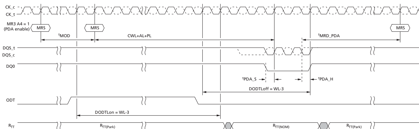
Figure 56: PDA Operation Enabled, BC4
