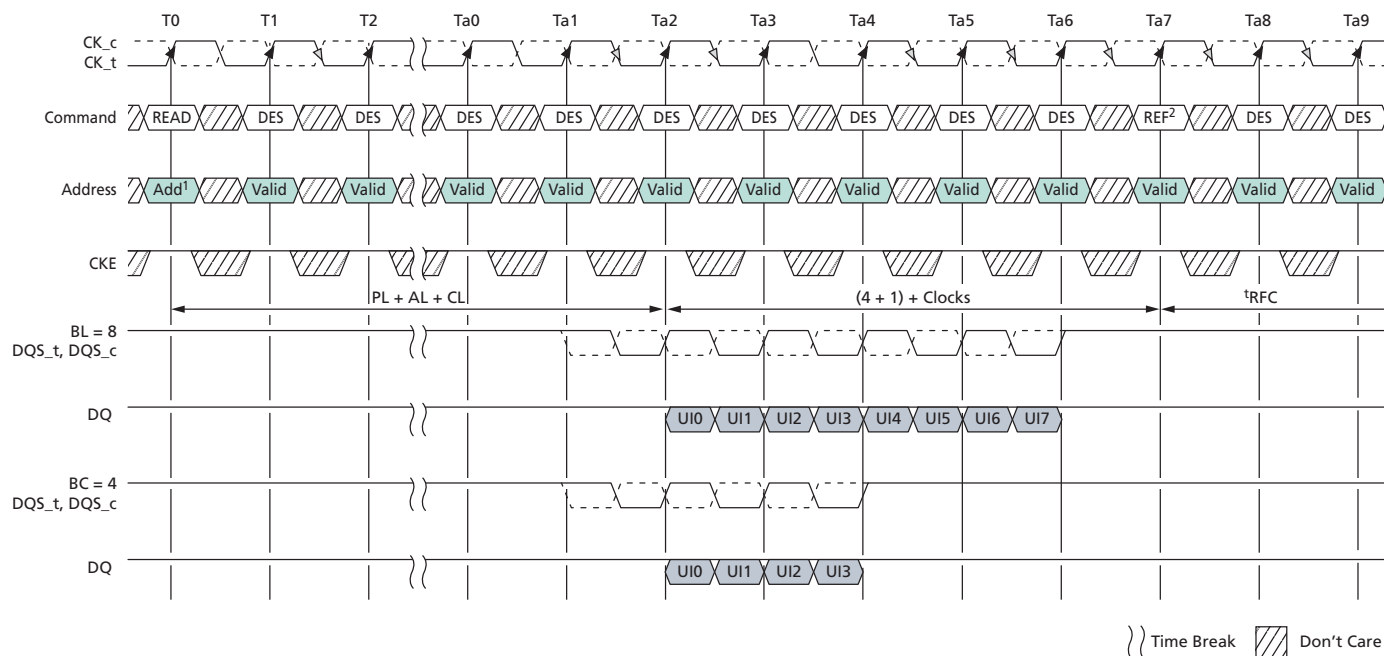
Figure 35: READ-to-REFRESH Timing
