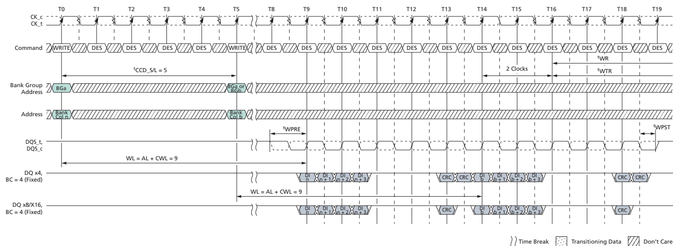
Figure 187: Consecutive WRITE (BC4-Fixed) with 1 st CK Preamble and Write CRC in Same or Different Bank Group
