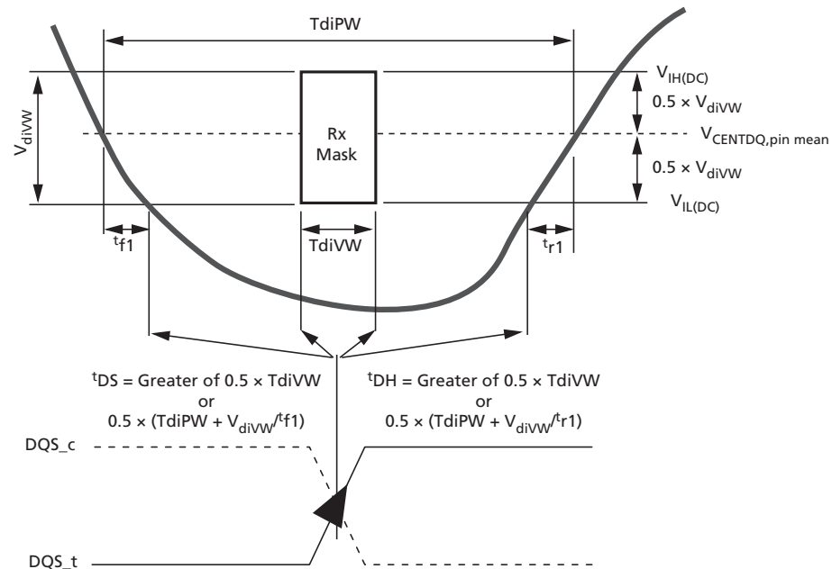
Figure 203: Rx Mask Relative to t DS/ t DH
