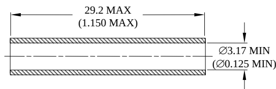
4. INSULATION SLEEVE, Qty: 2
