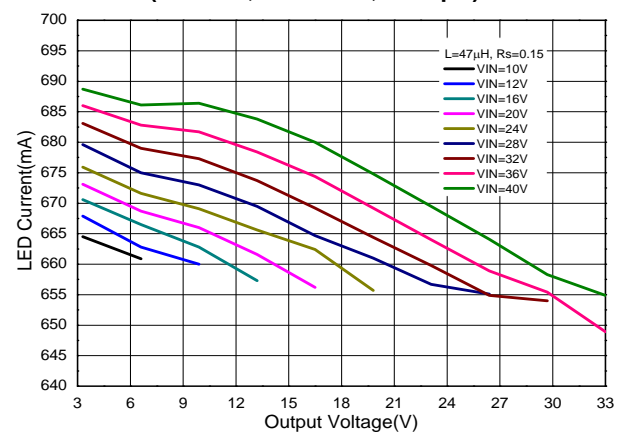
LED Current vs. Output Voltage (TSOT25, R_s = 0.15\Omega , L = 47\mu\text{H} )
