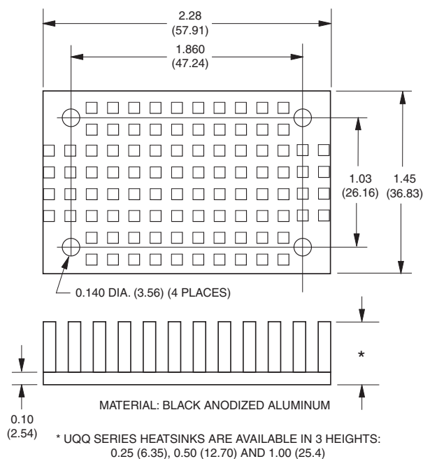
Figure 8. Optional Heatsink
