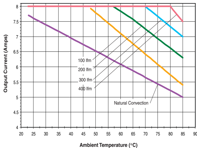
UQQ-12/8-Q48P Maximum Current Temperature Derating
