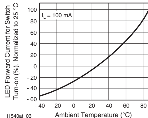
Fig. 4 - LED Current for Switch Turn-on vs. Temperature
