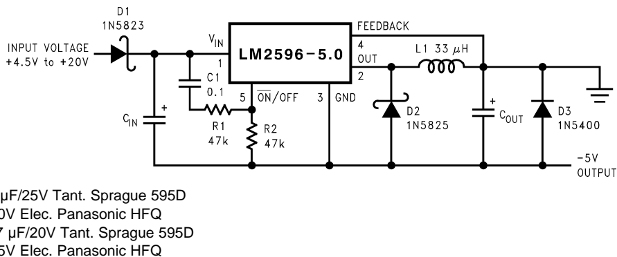
Figure 37. Inverting -5V Regulator with Delayed Startup
