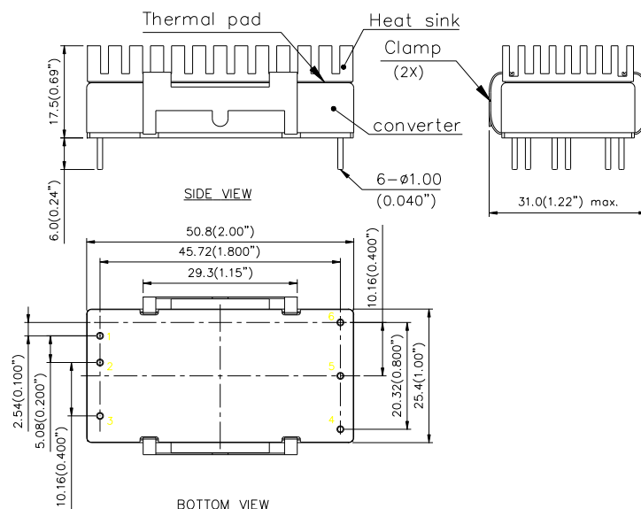
Mechanical Dimensions
