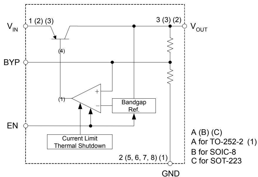
Figure 3. Functional Block Diagram of AP2213
