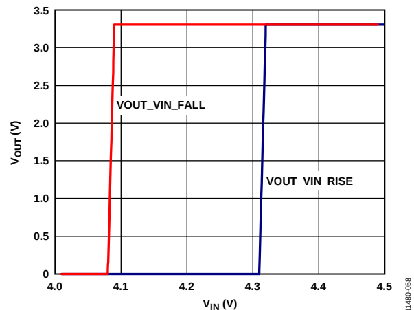
Figure 58. Typical UVLO Hysteresis, V_{OUT} = 3.3\text{ V}
