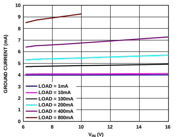
Figure 17. Ground Current vs. Input Voltage ( V_{IN} ), ADM7151-04, V_{OUT} = 5V
