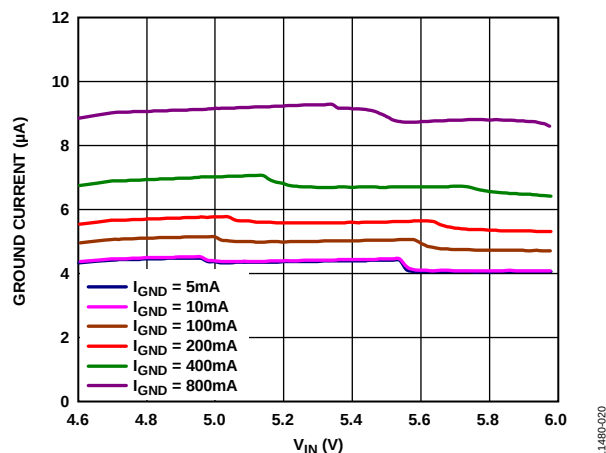
Figure 20. Ground Current vs. Input Voltage ( V_{IN} ) in Dropout, ADM7151-04, V_{OUT} = 5V
