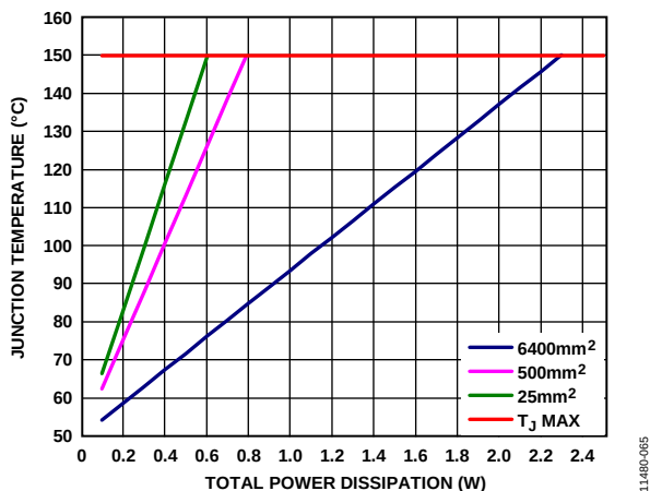
Figure 65. Junction Temperature vs. Total Power Dissipation for the 8-Lead SOIC, T_A = 50^\circ\text{C}
