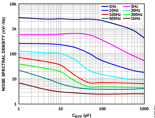
Figure 53. Noise Spectral Density vs. C_{\text{BYP}} for Different Frequencies
