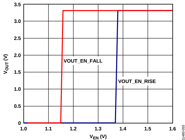
Figure 55. Typical V_{OUT} Response to EN Pin Operation, V_{OUT} = 3.3\text{ V} , V_{IN} = 5\text{ V}
