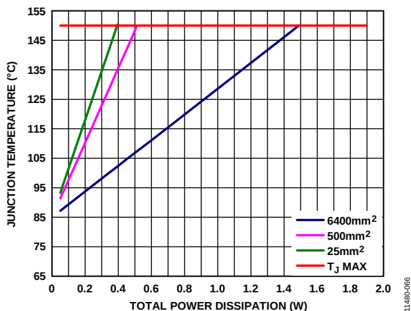
Figure 66. Junction Temperature vs. Total Power Dissipation for the 8-Lead SOIC, T_A = 85^\circ\text{C}
