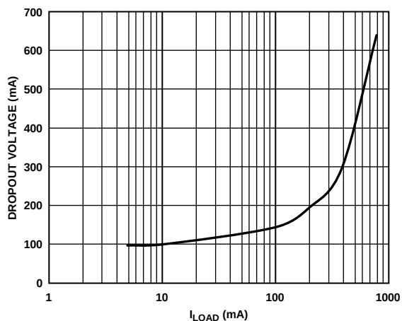
Figure 18. Dropout Voltage vs. Load Current ( I_{LOAD} ), ADM7151-04, V_{OUT} = 5V
