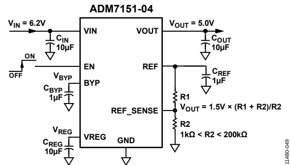
Figure 49. Typical Adjustable Output Voltage Application Schematic
