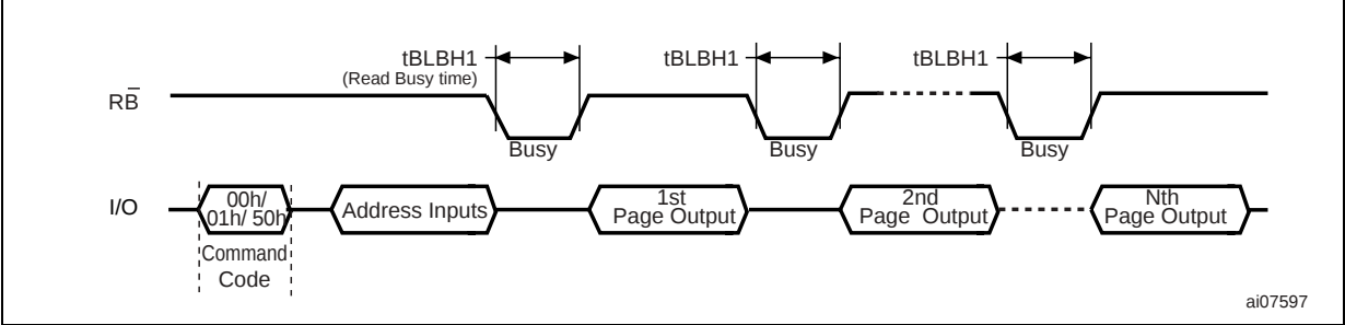
Figure 15. Sequential Row Read Operations
