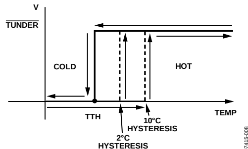
Figure 20. ADT6401 TUNDER Transfer Function
