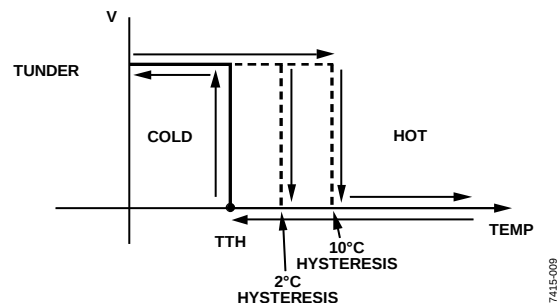
Figure 21. ADT6402 TUNDER Transfer Function
