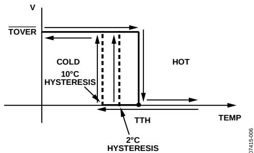
Figure 18. ADT6401 TOVER Transfer Function
