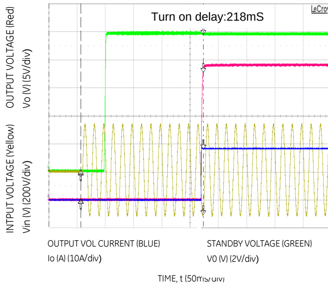
Figure 5. Typical Start-up ( V_{IN} = 230\text{Vac} , Full Load).
