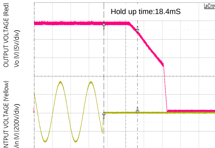
Figure 7. Typical Hold-up waveforms ( V_{IN} = 230\text{V} , 100% load)
