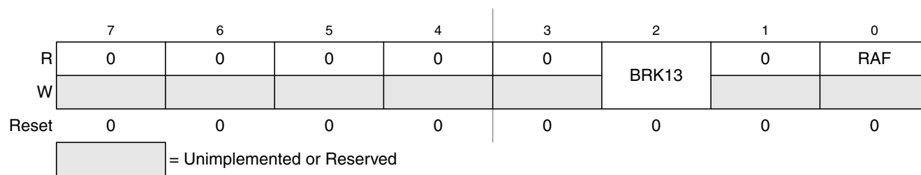
Figure 11-9. SCI Status Register 2 (SC1xS2)
