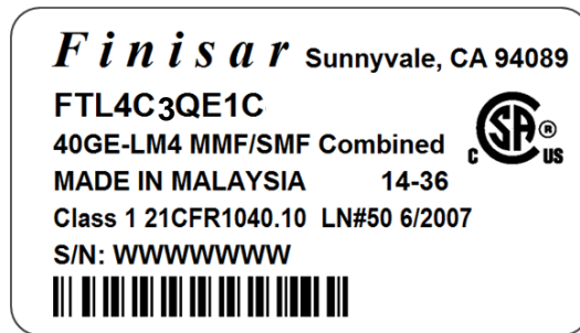
Figure 3 – FTL4C3QE1C label
