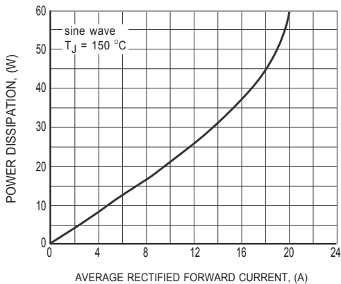
FIG.2 POWER DISSIPATION
