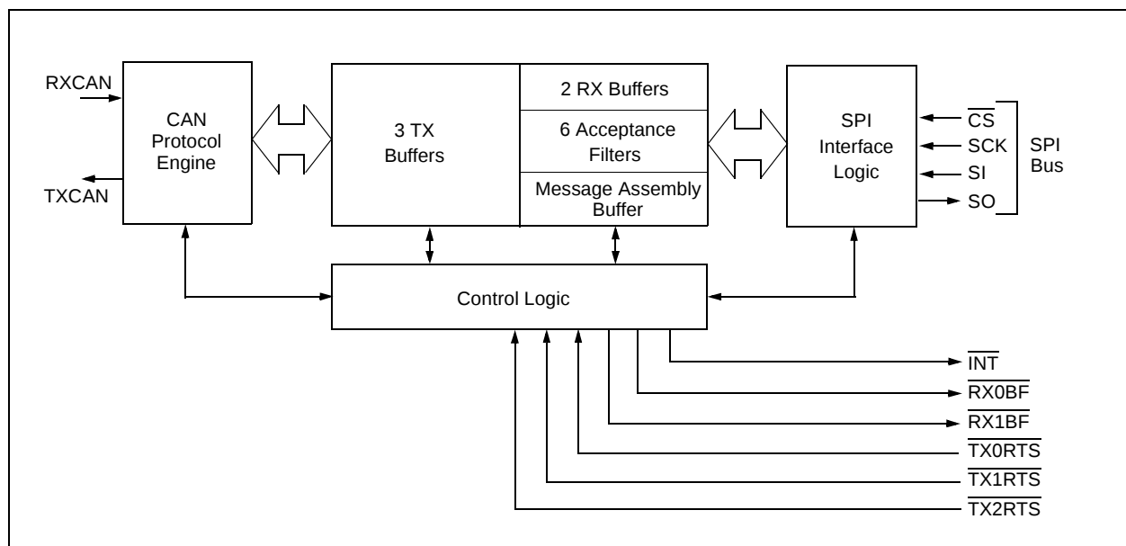
FIGURE 1-1: Block Diagram
