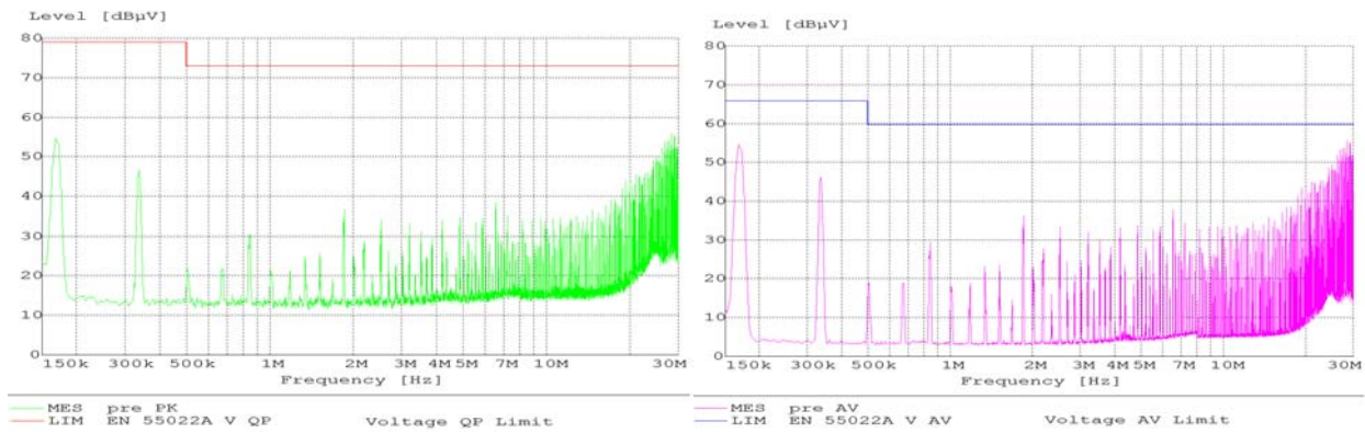
Figure 23. EMC Filter
