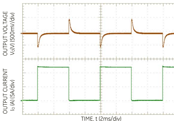
Figure 6. Dynamic Load Change Transient Response from 0 % to 75% to 0% of Full Load at Room Temperature and 48 Vin; 2.0A/uS, C_{o,ext} = 880\mu F .
