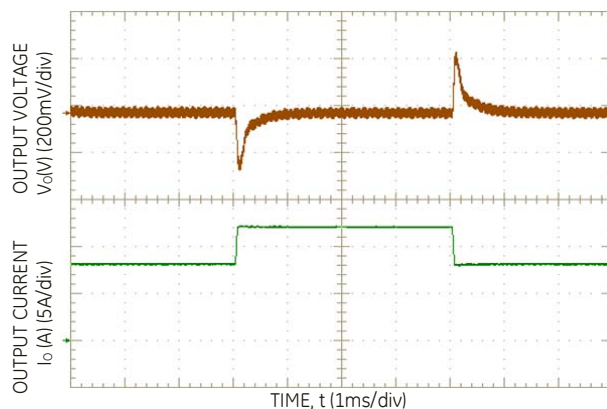
Figure 3. Dynamic Load Change Transient Response from 50% to 75% to 50% of Full Load at Room Temperature and 48 Vin; 0.1A/uS, C_{o,ext} = 470\mu F .
