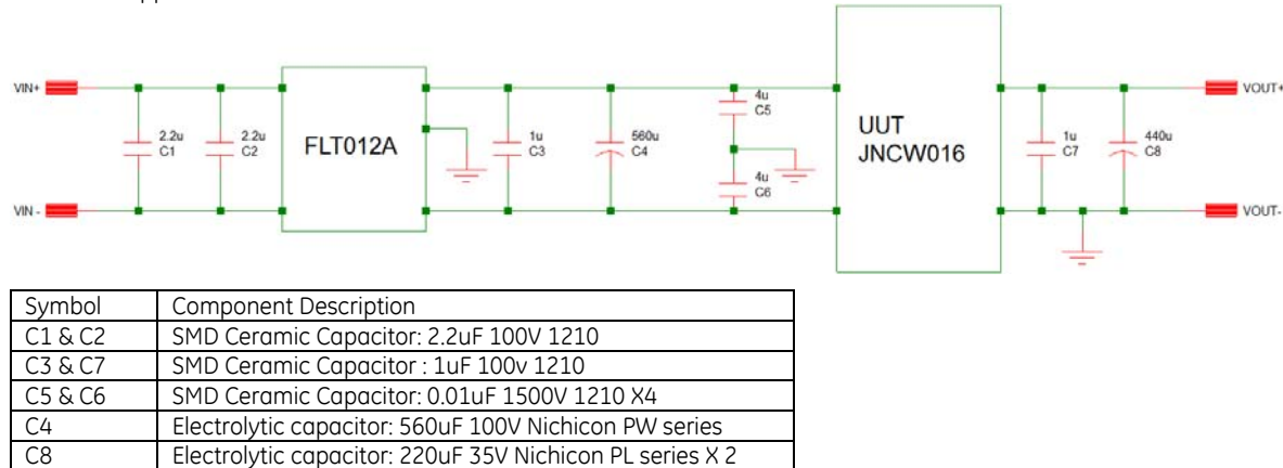
Figure 23. EMC Filter
