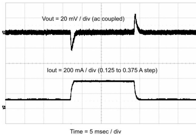
Figure 52. Load Transient
