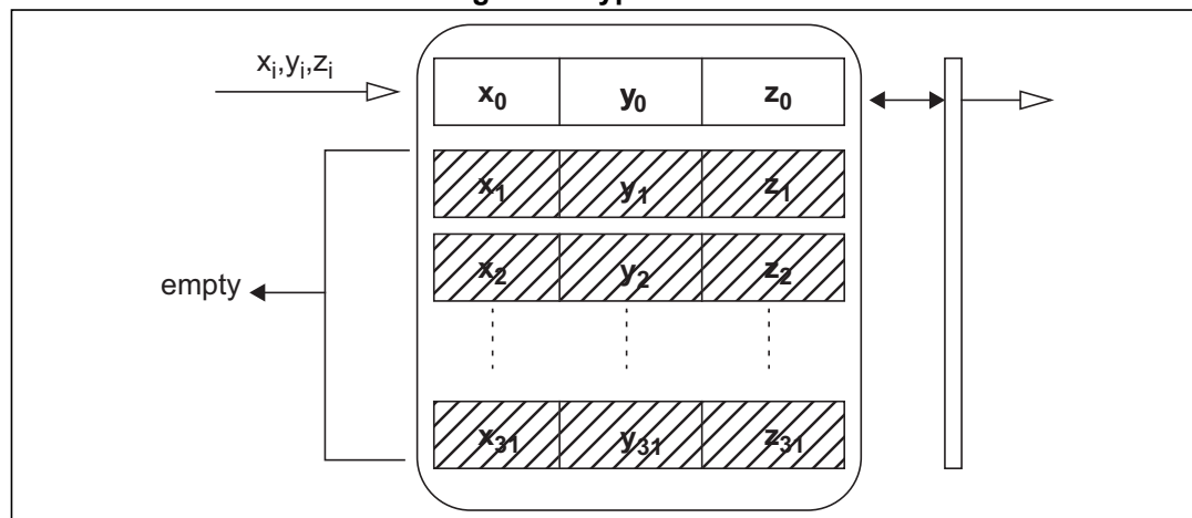
Figure 9. Bypass mode
