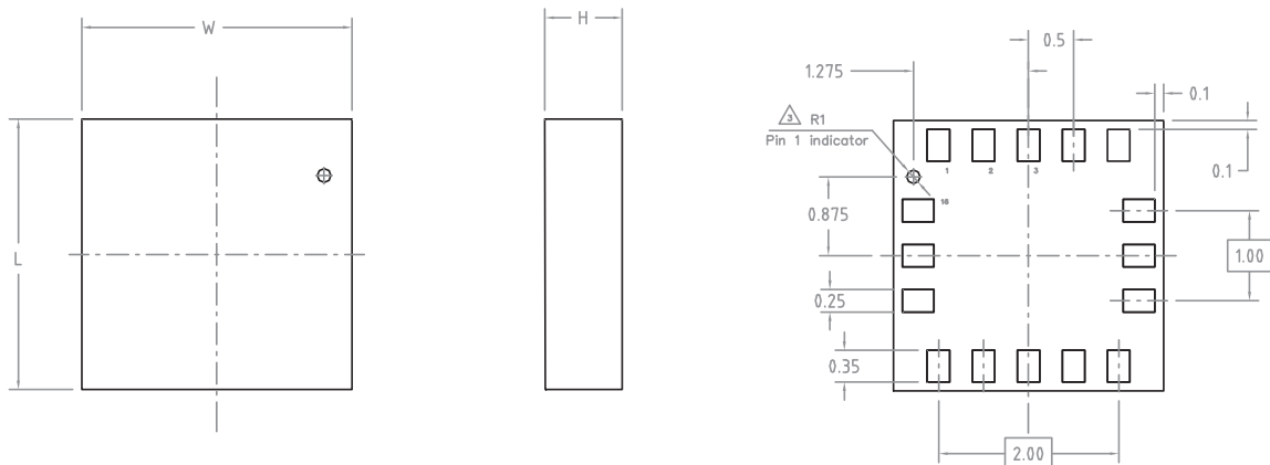
Figure 24. LGA 3x3x0.86 16L package outline and dimensions
