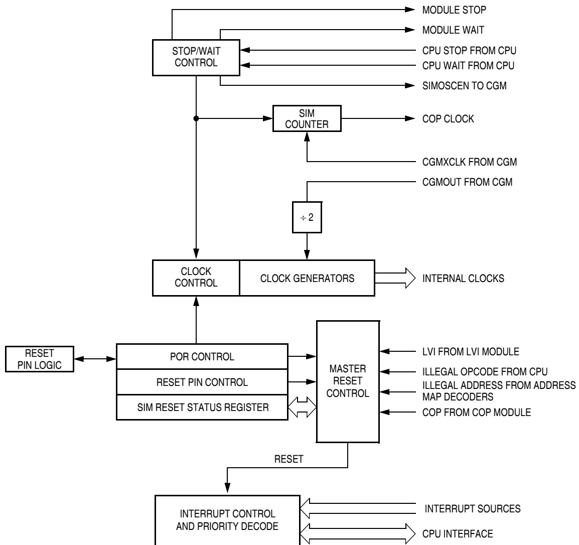
Figure 9-1. SIM Block Diagram
