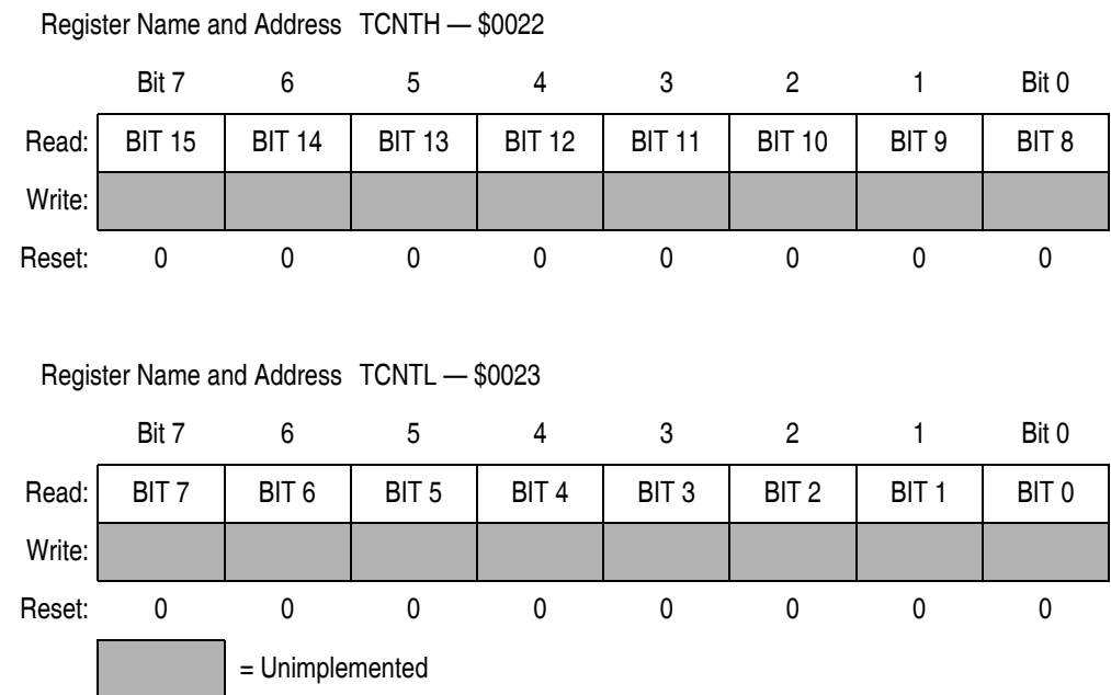
Figure 16-4. TIM Counter Registers (TCNTH and TCNTL)
