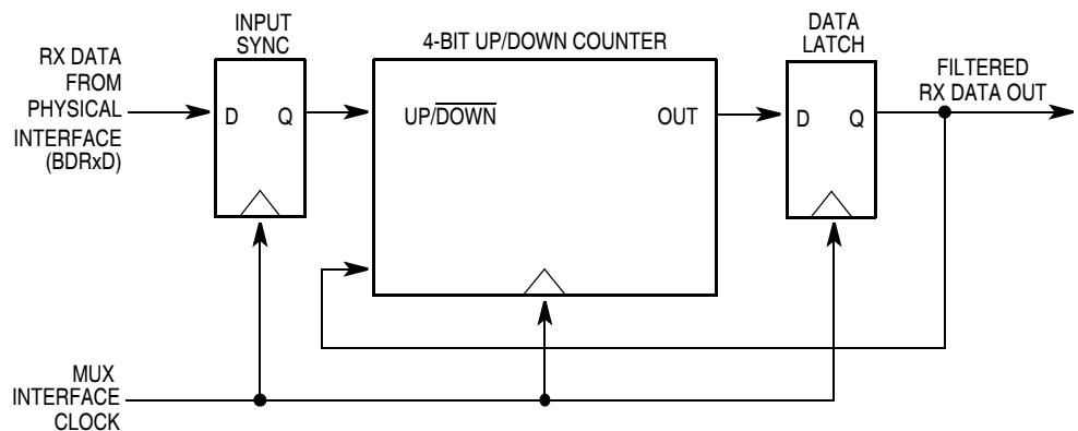
Figure 20-4. BDLC Rx Digital Filter Block Diagram
