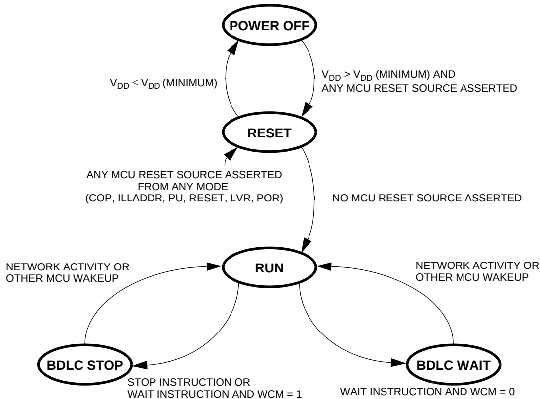
Figure 20-2. BDLC Operating Modes State Diagram
