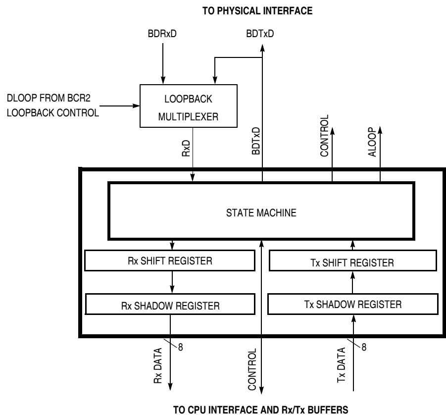
Figure 20-13. BDL Protocol Handler Outline
