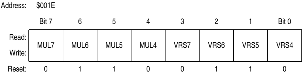
Figure 8-5. PLL Programming Register (PPG)
