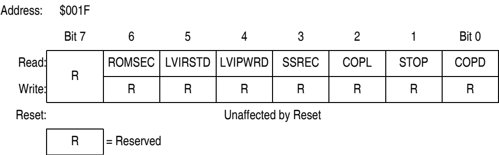
Figure 5-1. Mask Option Register (MOR)
