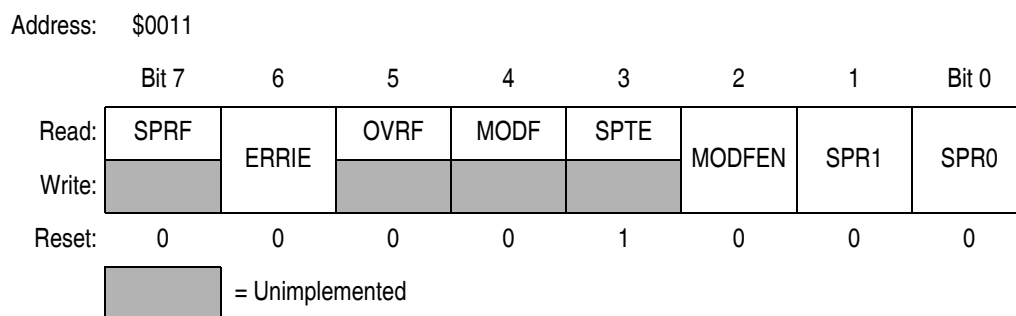
Figure 18-13. SPI Status and Control Register (SPSCR)
