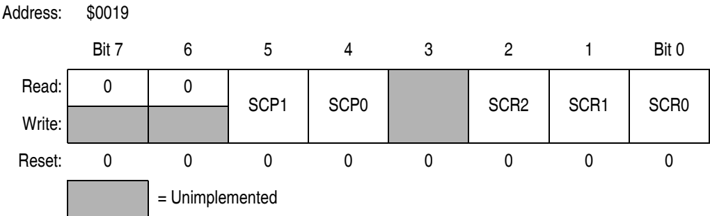
Figure 17-13. SCI BAUD Rate Register (SCBR)
