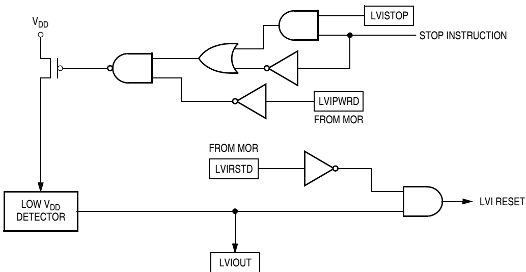
Figure 10-1. LVI Module Block Diagram
