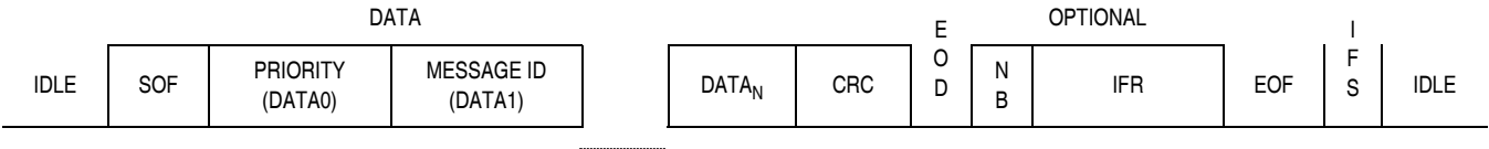
Figure 20-5. J1850 Bus Message Format (VPW)
