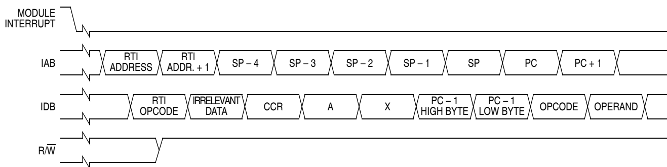
Figure 9-9. Hardware Interrupt Recovery Timing
