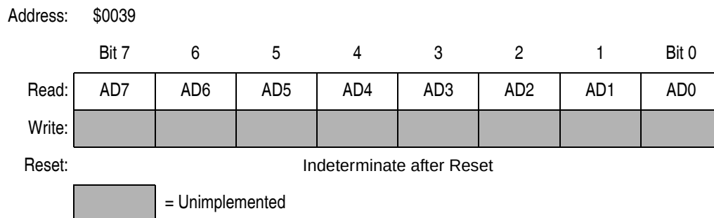
Figure 19-3. ADC Data Register (ADR)
