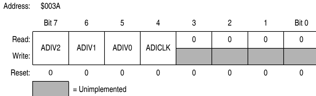
Figure 19-4. ADC Input Clock Register (ADICLK)
