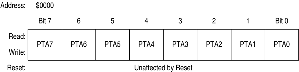
Figure 15-1. Port A Data Register (PTA)
