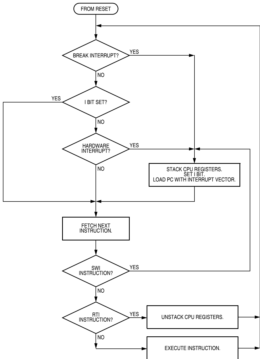
Figure 9-8. Interrupt Processing
