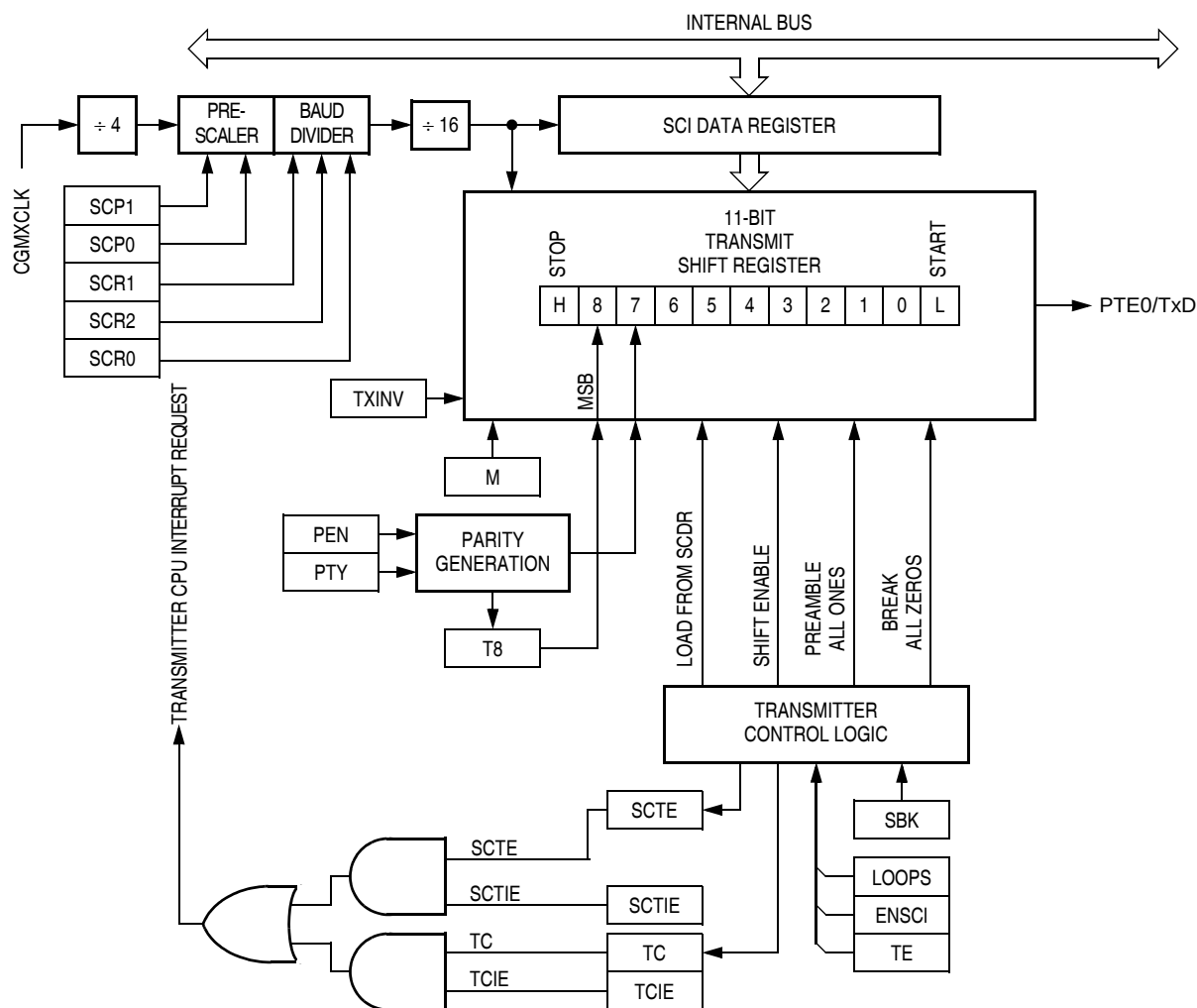
Figure 17-3. SCI Transmitter
