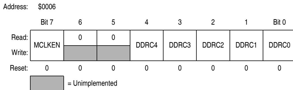
Figure 15-8. Data Direction Register C (DDRC)
