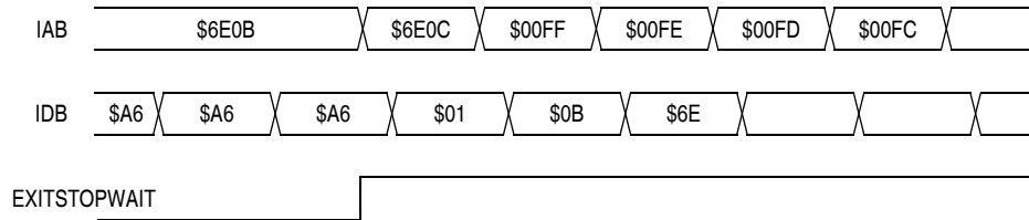
Figure 9-12. Wait Recovery from Interrupt or Break
