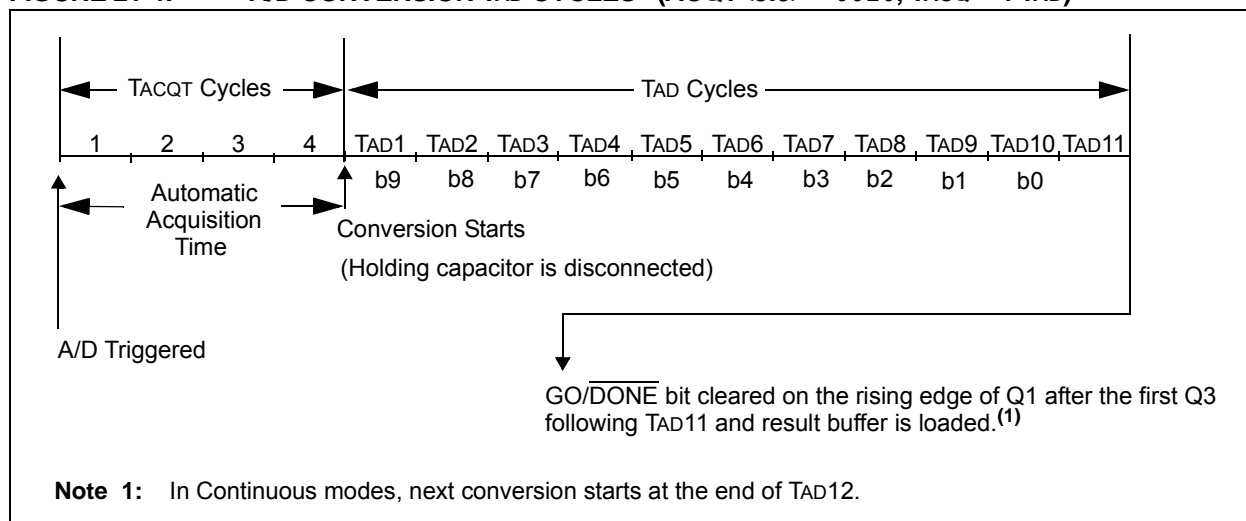
FIGURE 21-4: A/D CONVERSION TAD CYCLES ( \text{ACQT}<3:0> = 0010 , \text{TACQ} = 4 \text{ TAD} )
