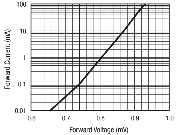
Figure 2. DC Characteristics
