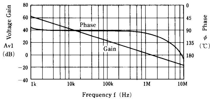
AMP#A Loop Gain, Phase vs. Frequency
