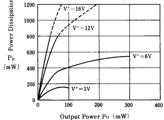
Power Dissipation vs. Output Power
