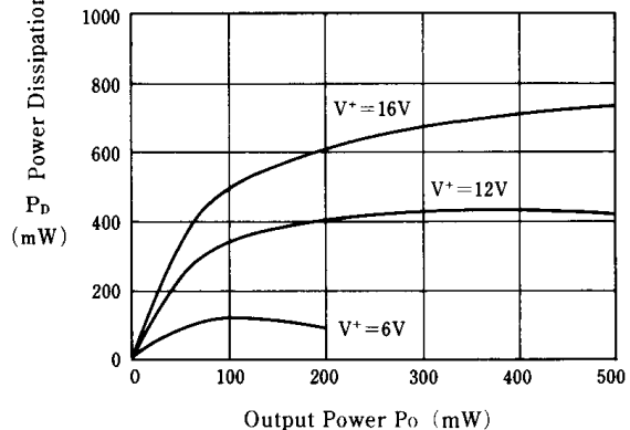
Power Dissipation vs. Output Power
