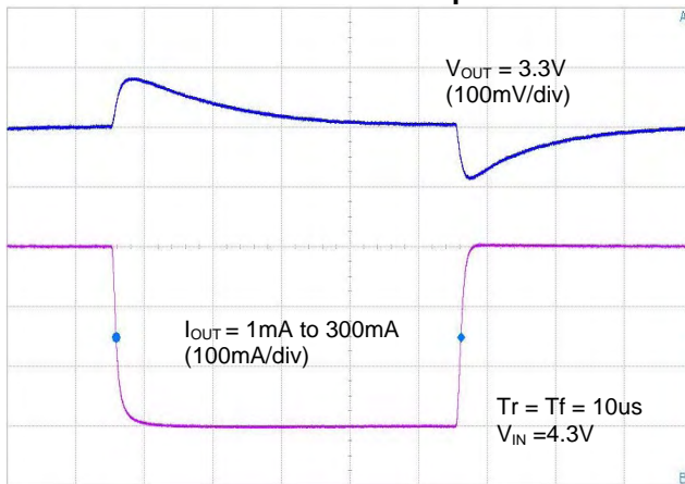
Time (100us/div)
