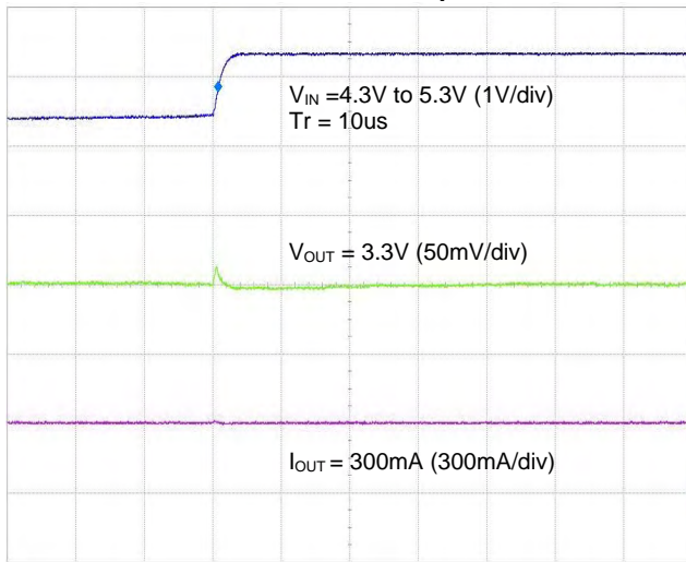
Time (50us/div)
