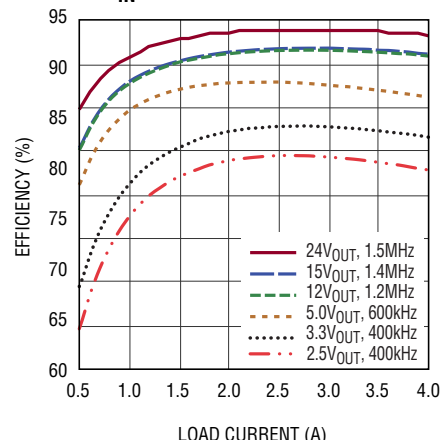
Efficiency vs Load Current at 48V IN , Forced Continuous Mode
