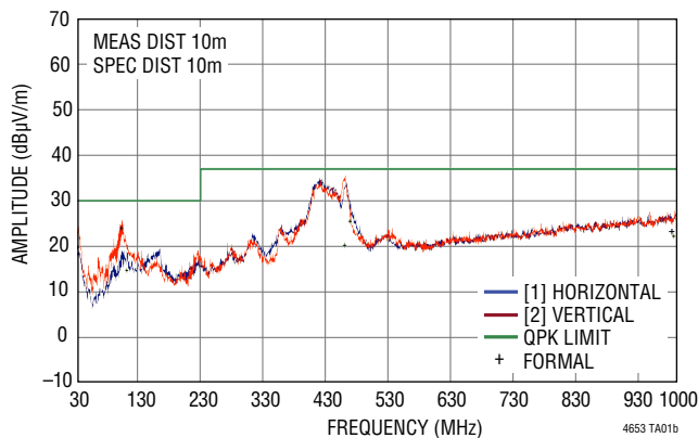
Radiated Emission Scan in a 10m Chamber LTM4653 Delivering 24V OUT at 3.5A, from 48V IN
