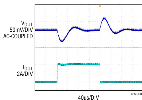
1V Transient Response, 24V IN
