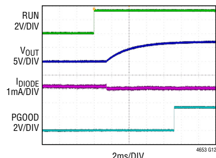
Start-Up, Pre-Bias
